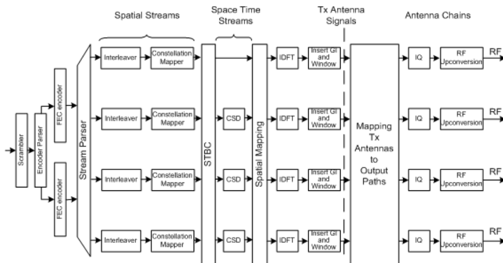
Fig. 2-2: IEEE 802.11 n Transmission chain
