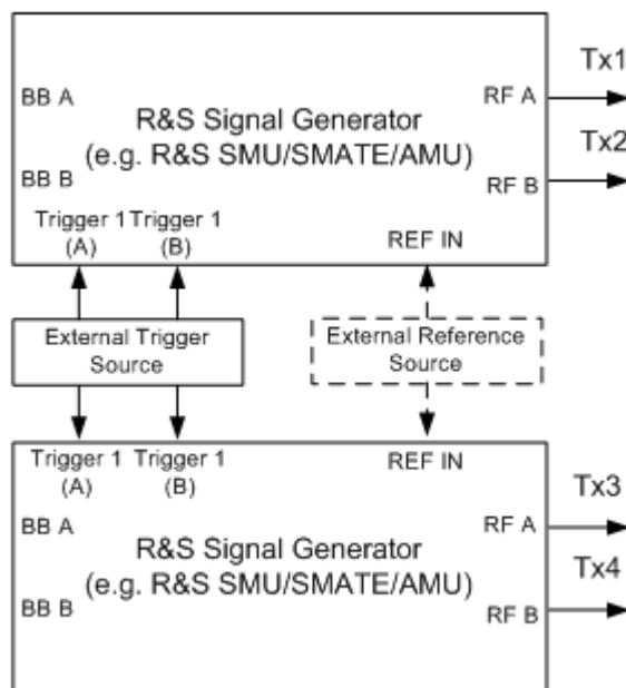
Fig. 2-3: Connecting two two-path R&S Signal Generators for the generation of 4xN MIMO WLAN-N signal
