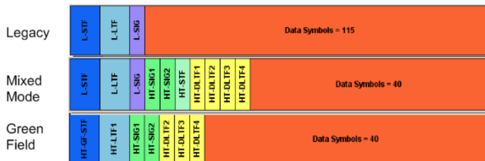
Fig. 2-1: PLCP Packet format for IEEE 802.11n
